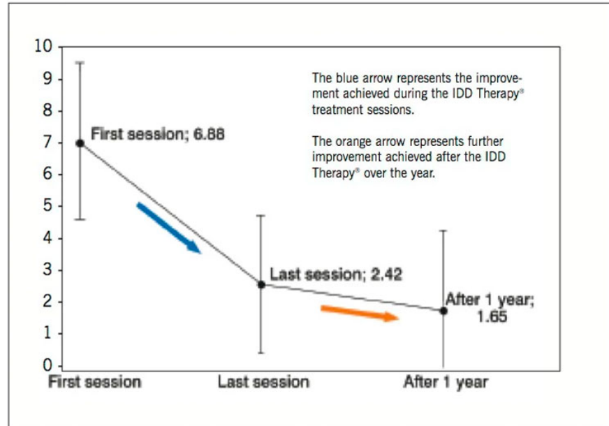
FIGURE 1. The chart shows mean NPS of 6.88 at the beginning of IDD Therapy® treatment after the completion of treatment the mean NPS is reduced to 2.42 (last session). After a duration of one year the patients continue to improve and the mean NPS is 1.65.
